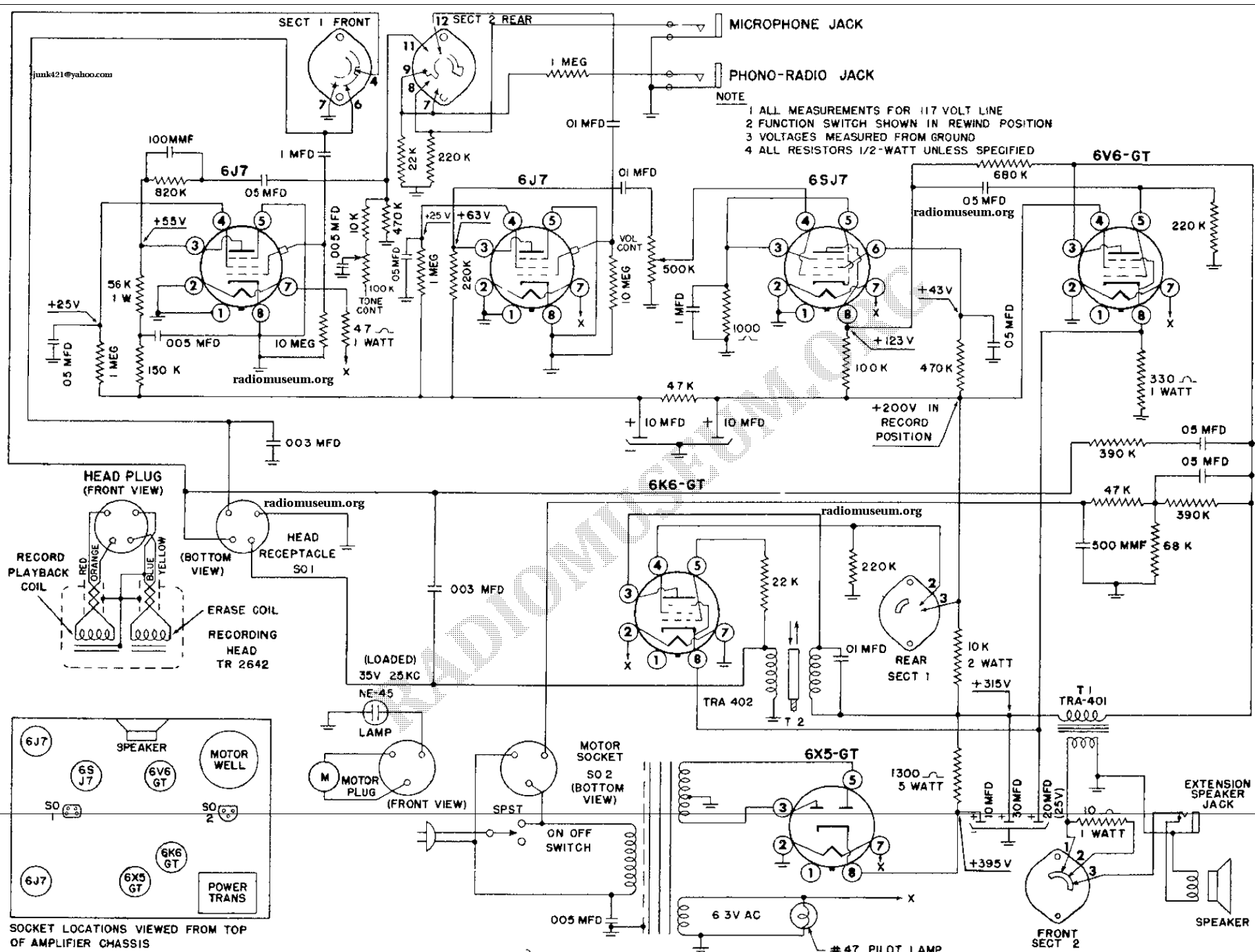
FIG 16 - Schematic Circuit Diagram
