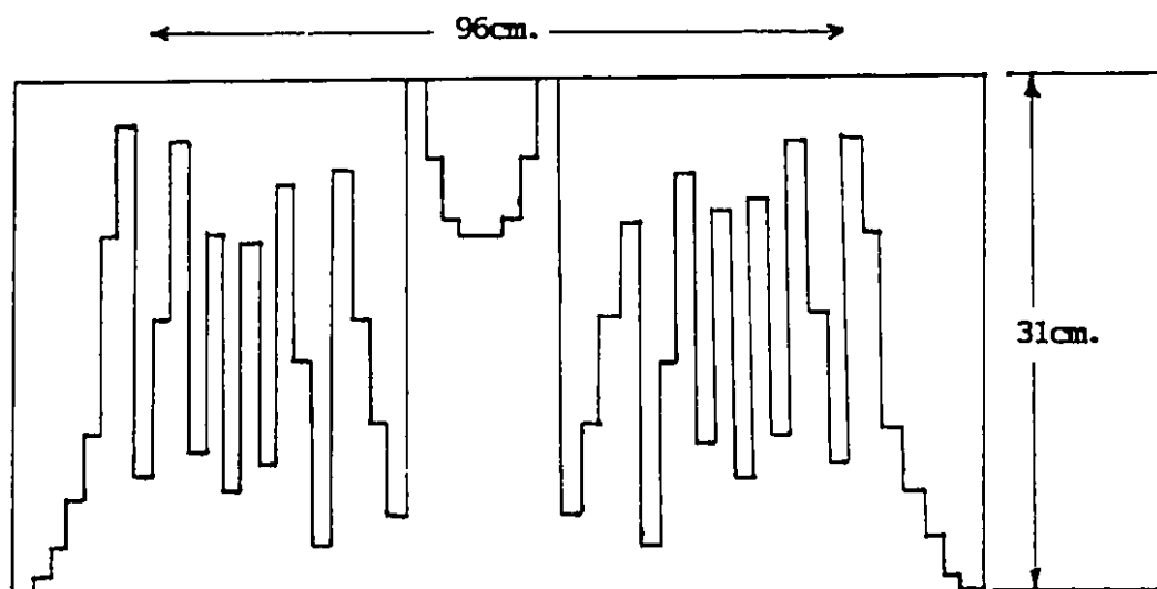
(6-5) Top view of diffuser module showing grating sequence pattern.
